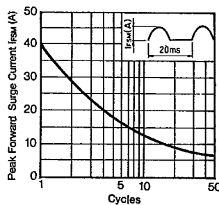
IFSM Characteristics
